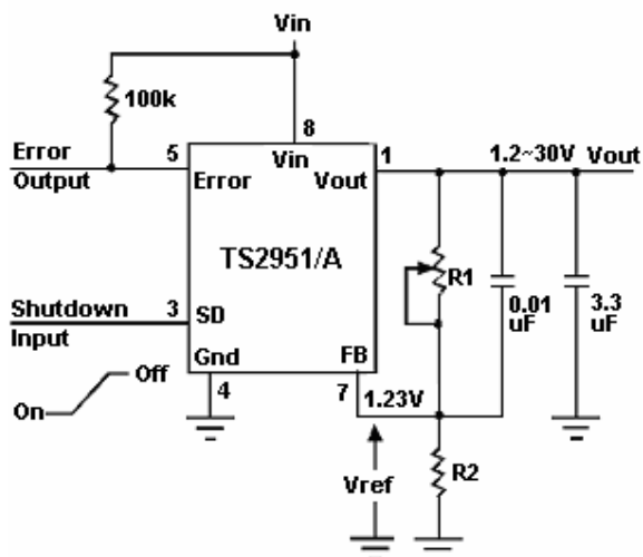
Figure 2. Adjust Voltage
