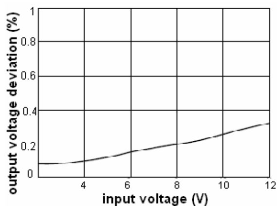
Figure 4: line regulation
