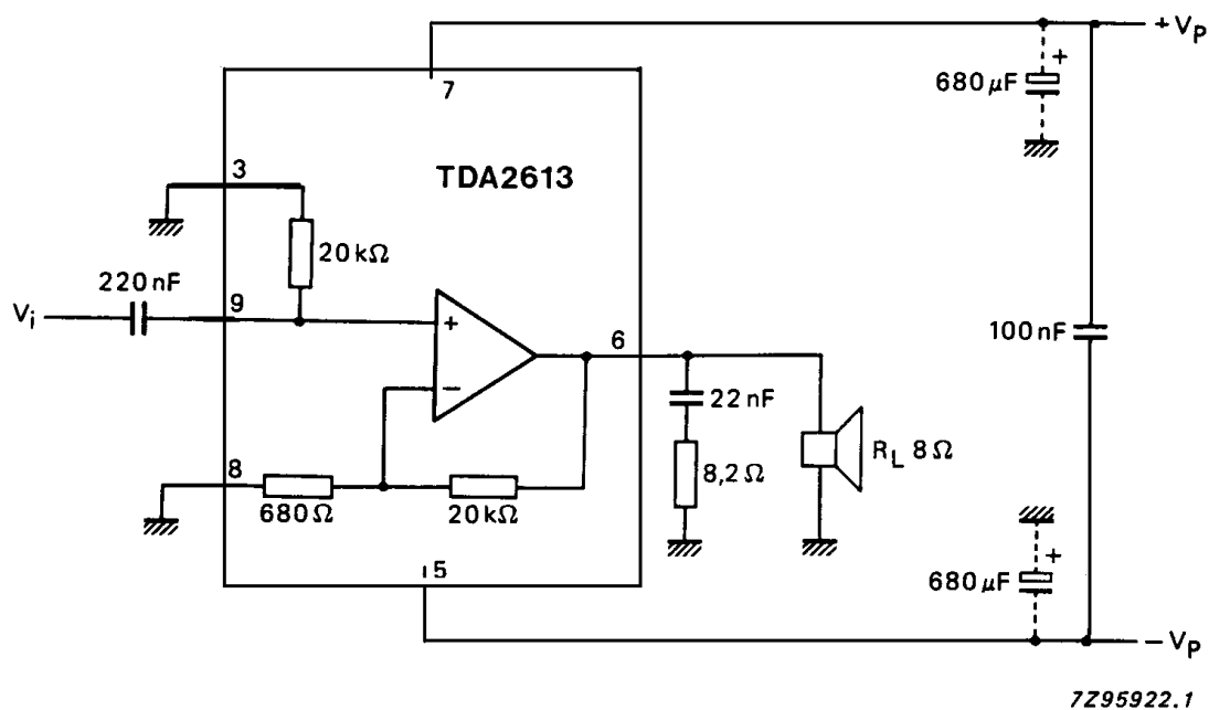
Fig.3 Test and application circuit; symmetrical power supply.
