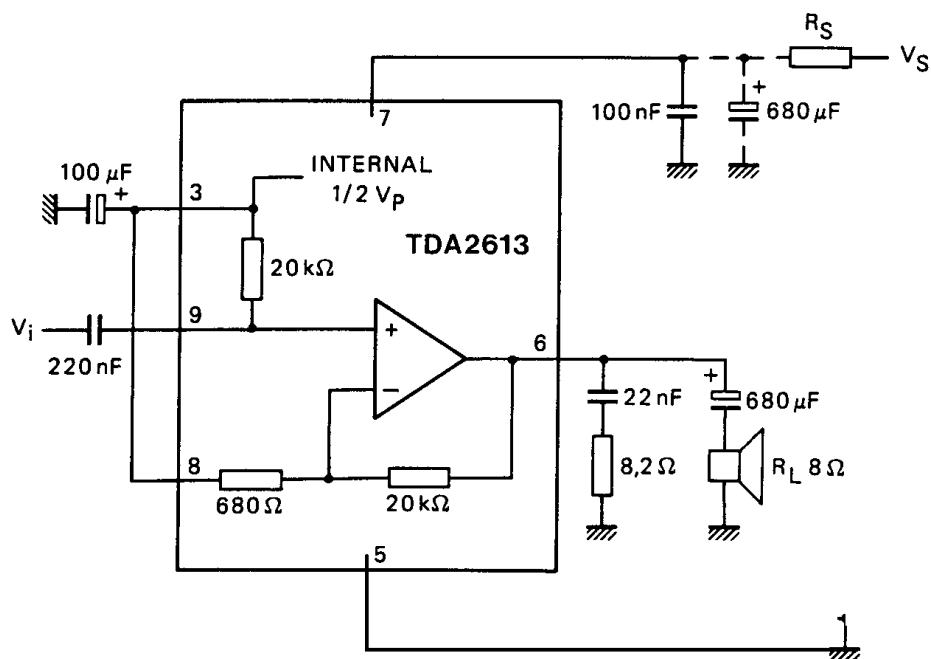
Fig.4 Test and application circuit; asymmetrical power supply.
