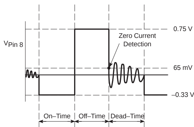
Figure 31. Demagnetization Detection
