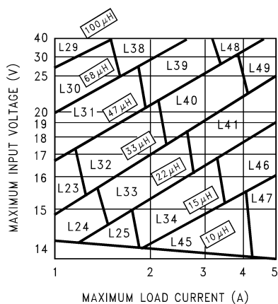
Figure 23. LM2678-12
