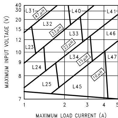
Figure 22. LM2678-5.0
