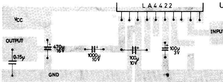
Printed Circuit Pattern (22 x 65mm 2 , Cu-foiled side)
