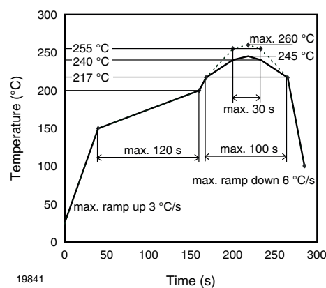
Fig. 15 - Lead (Pb)-free Reflow Solder Profile According to J-STD-020 for SMD-8 Devices
