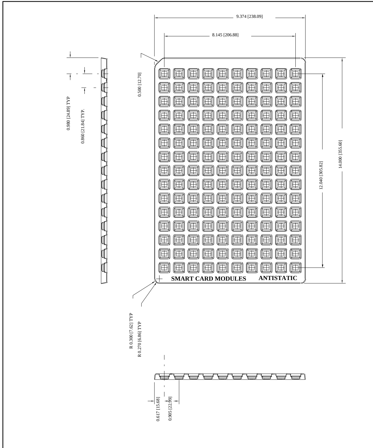
FIGURE 9-1: TRAY DIMENSIONS
